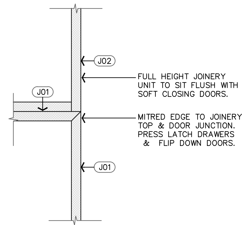
DETAIL DRAWING
